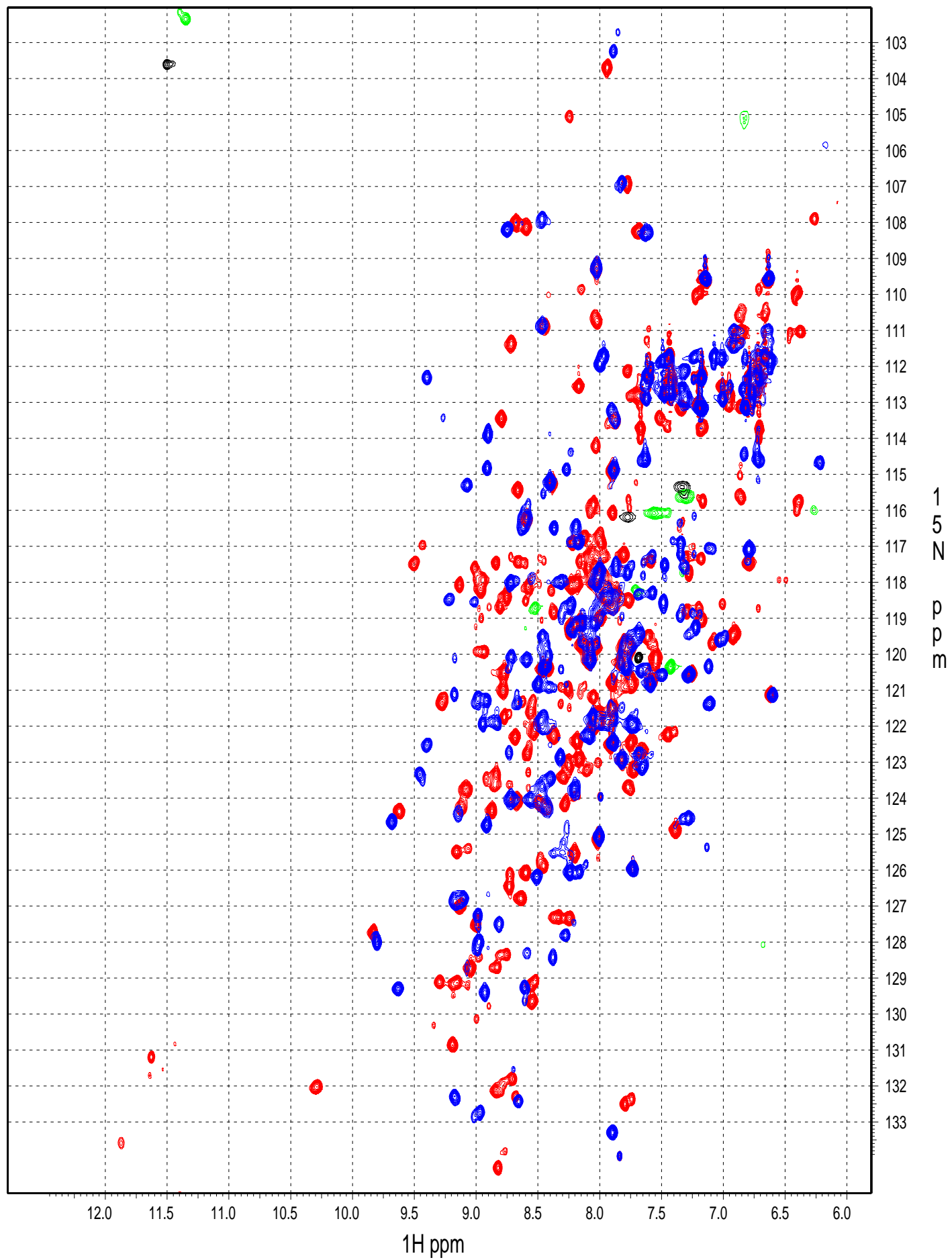
^{15}\text{N} Pixj Pr (red-pos./green-neg.) vs. Pfr (blue-pos./black-neg.) @ 600 MHz 25 C
